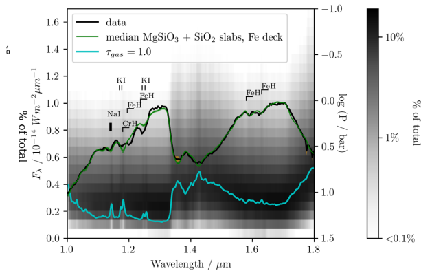
Figure 9. Comparison of our preferred model J and H band spectrum with the data for 2M2224-0158. The 1\sigma spread in the model distribution is shown in green shading, and the errors for the data are shaded in orange. Both are mostly covered by the line width except in a few places. Features responsible for regions of particularly poor fit are annotated. Also plotted, with its y-scale on the right-hand side, is the contribution function. The \tau = 1 line for gas-phase absorption is indicated with a cyan line.
