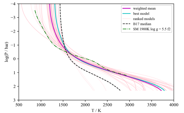
Figure 6. A comparison of retrieved thermal profiles under different cloud model assumptions. Models other than our preferred model are plotted with line opacities proportional to (1/\log(\Delta BIC)) . The preferred model profile and the likelihood weighted mean of the profiles are indicated. Also plotted are the median retrieved profile for 2M2224-0158 from B17, and an example self-consistent grid model that closely matches our retrieved T_{\text{eff}} and \log g .
