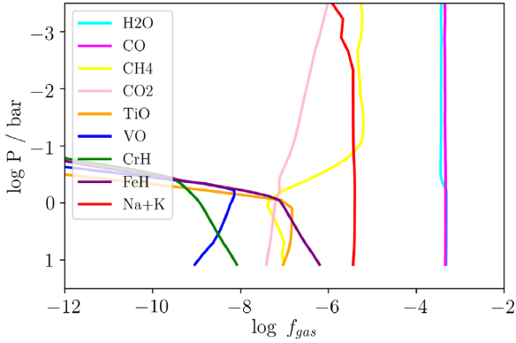
Figure 1. Predicted gas fractions ( f_{\text{gas}} ) from our thermochemical grid calculated along a grid model T_{\text{eff}} = 1700 K \log g = 5.0 thermal profile.
