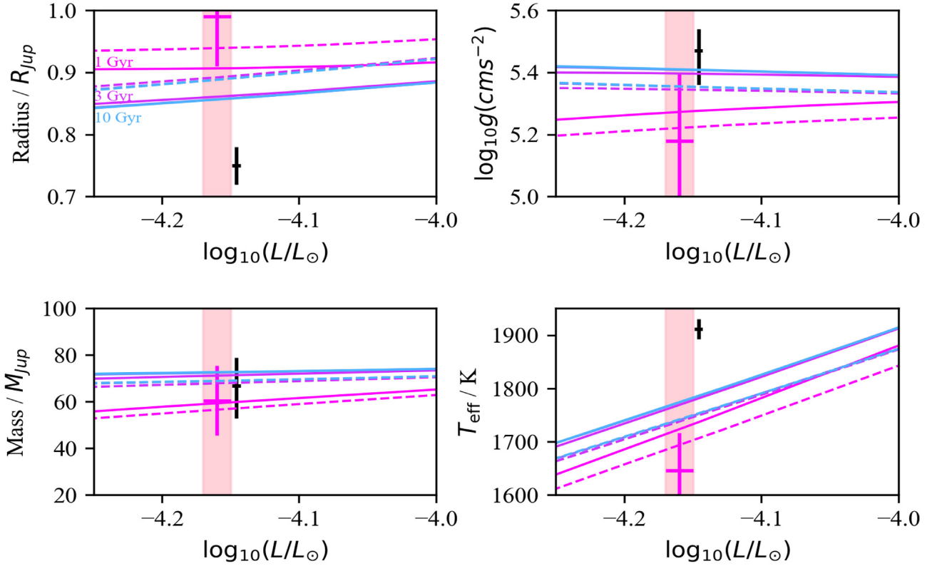
Figure 5. Comparisons of our retrieved and extrapolated values for bulk properties of 2M2224-0158 with the empirical bolometric luminosity calculated by Filippazzo et al. (2015; shaded pink) and Sonora-Bobcat cloud-free evolutionary models (Marley & Saumon 2020) for solar metallicity (solid lines) and [M/H] = +0.5 (dashed lines). Magenta error bars are the semi-empirical values from Filippazzo et al. (2015), which used a combination of DUSTY00 (Chabrier et al. 2000), SMHC08 (Saumon & Marley 2008), and f_{\text{sed}} = 2 Saumon & Marley (2008) isochrones. Our retrieval based estimated values are indicated with black error bars. Their derivation is described in Section 5.3.
