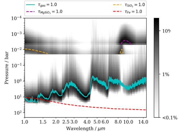
Figure 8. Contribution function for a spectrum based on the maximum likelihood retrieved parameters for the top-ranked model. The contribution function in an atmospheric layer, lying between pressures P_1 and P_2 is defined as C(\lambda, P) = \frac{B(\lambda, T(P)) \int_{P_1}^{P_2} d\tau}{\exp \int_{P_0}^{P_2} d\tau} . \tau = 1 lines are included for gas phase opacities and each of our cloud species.
