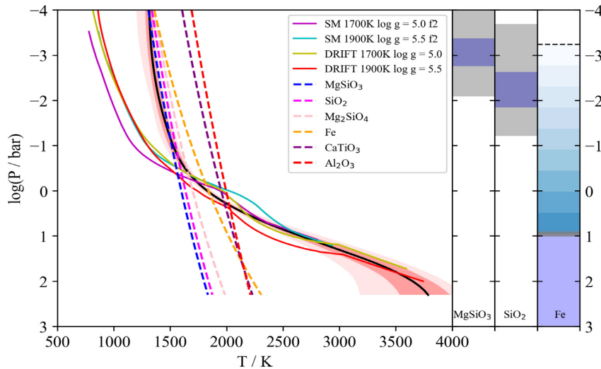
Figure 3. Retrieved thermal profile (black line, pink shading for 1\sigma and 2\sigma intervals) and cloud pressures for 2M2224-0158, plotted with self-consistent model profiles from the Drift-Phoenix (prefixed Drift, Helling et al. 2008) and Saumon & Marley grids (prefixed SM, Saumon & Marley 2008). Also plotted are phase-equilibrium condensation curves for various potential condensates. The clouds pressures are indicated in bars to the left of the P/T profile. Blue shading indicates the median cloud location for the two slab cloud, with grey shading indicating the 1\sigma range. The deck cloud is furthest to the right, with the uniform blue shading indicating the optically thick extent of the cloud deck, and grey shading the 1\sigma interval for the \tau = 1 location. Graduated shading shows the range over which the deck cloud optical depth drops to 0.5.
