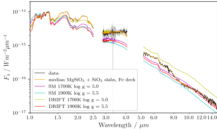
Figure 2. Maximum likelihood retrieved model spectrum for the top-ranked model overlaid with the data. The grey shading indicates the uncertainty in the data. Pink shading indicates the 95 per cent confidence interval in the retrieval, and is mostly hidden by the line weight. Self-consistent grid models are shown for comparison, and are scaled to match the J band flux in the observed spectrum.
