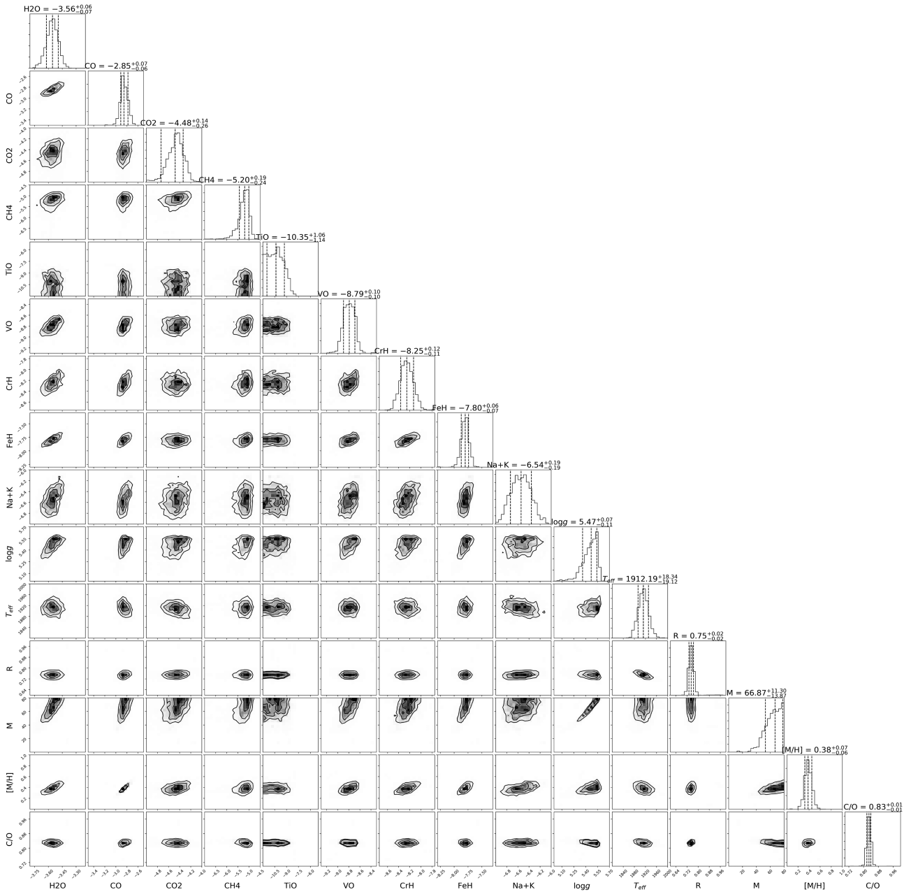
Figure 4. Corner plot showing the top-ranked model retrieved parameters that set the gaseous opacity in the atmosphere, \log g , along with derived values for radius, mass, atmospheric metallicity and C/O ratio, and extrapolated T_{\text{eff}} . See text for explanation of derived and extrapolated values.
