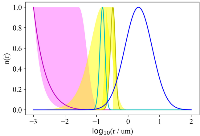
Figure 7. A comparison of particle-size distributions (normalized to have maximum values of 1) for our three retrieved cloud species, and the lognormal particle-size distribution used in the Saumon et al. (2007) self-consistent model grid. The coloured shading indicates the range of the 16th and 84th percentiles of the retrieved size distributions.
