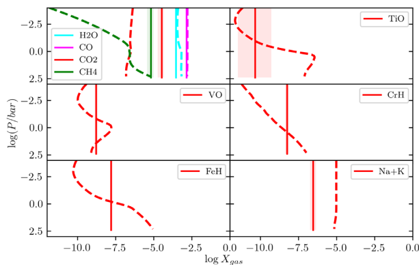
Figure 10. Retrieved gas fractions compared to predictions from our thermochemical grid for our estimated metallicity and C/O ratio. Equilibrium predictions are shown as dashed lines and are calculated for our estimated [M/H] and C/O values. The solid straight lines and shading show our median retrieved values and 16th to 84th percentiles, respectively.
